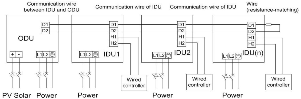
Fig. 25 Connection of power cord and communication wire for IDU and ODU (2)
